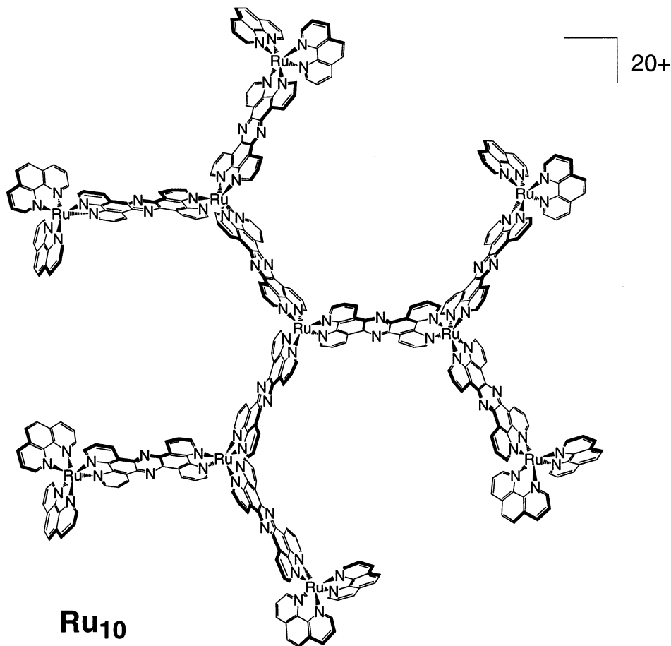
Fig. 10. Drawing of decanuclear dendrimer ( Ru 10 ).
